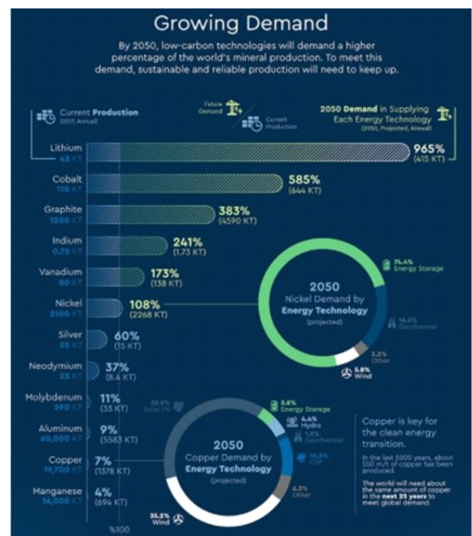
Minerals that will be key for expanding low-carbon technologies
